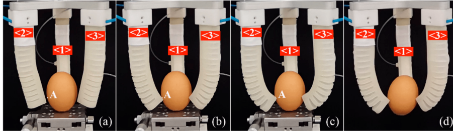
Figure 2.18: Pneumatic actuator grasping process of an egg [36]: (a) The soft actuator moves toward the egg when pneumatic module one is pressurized to 10 kPa, with module two remaining at zero pressure. (b) Contact between the tip of the soft actuator and the egg occurs when the pressure in module one is increased to 20 kPa and module two is set to 14.1 kPa. (c) The egg is securely pinched by the gripper when both module one and module two are pressurized to 20 kPa. (d) The egg is held firmly when the supporting platform is removed, indicating a stable grasp by the gripper.
