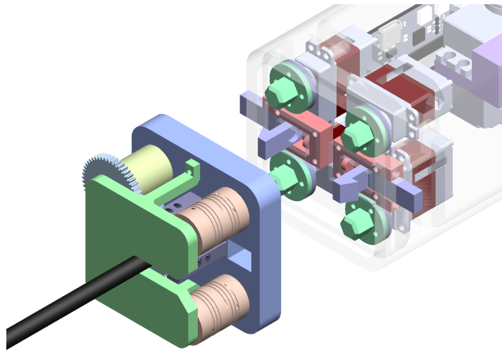
Figure 7.5: Motor Arrangement and Quick-Swap Mechanism
