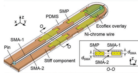
Figure 2.13: Shape Memory Alloy-Based Soft Gripper [31]
