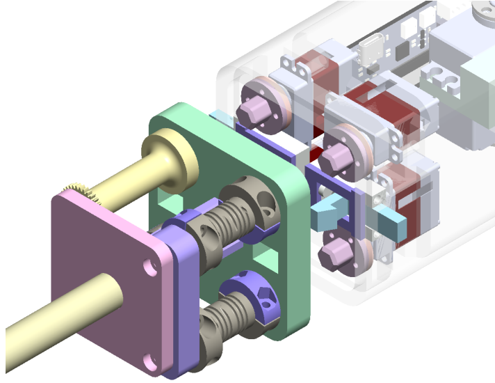
Figure 7.4: Motor Arrangement and Quick-Swap Mechanism
