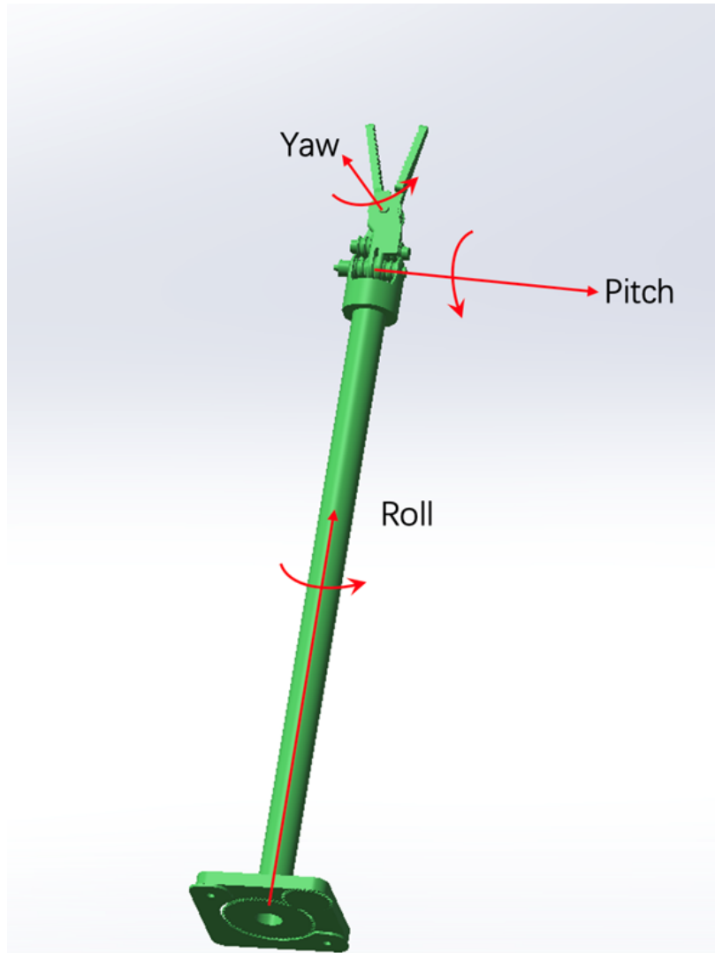
Figure 7.6: Denavit–Hartenberg coordinate frame definition for the manipulator
