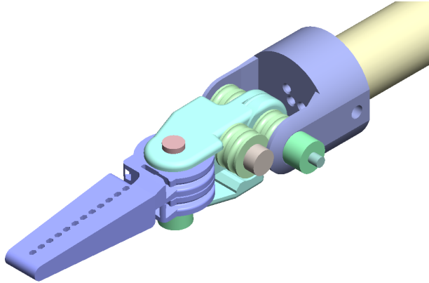
Figure 7.2: Tip Design for Cable Guidance
