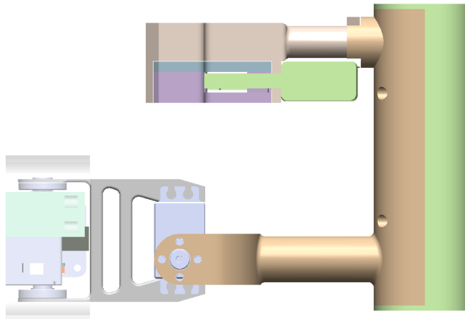
Figure 7.5: Input Module Design
