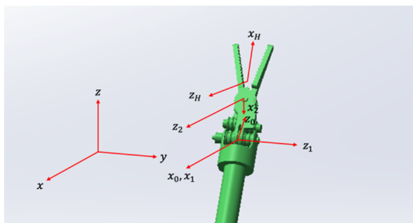
Figure 7.7: Alternative view of the D-H coordinate frames and joint axes
