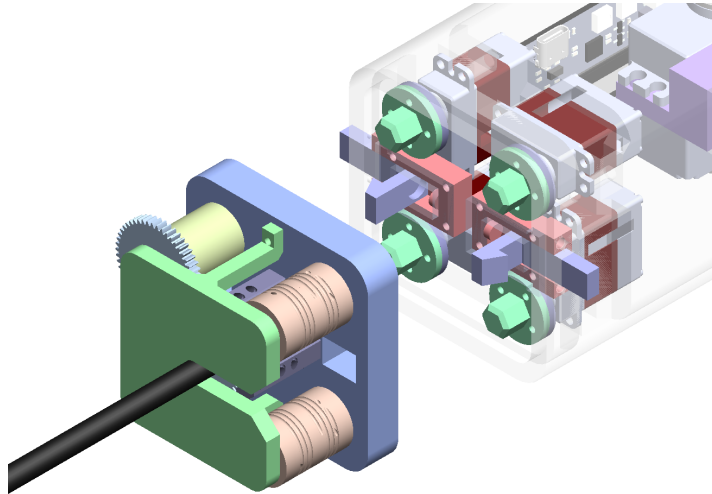
Figure 5.5: Motor Arrangement and Quick-Swap Mechanism
