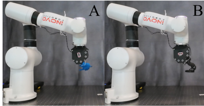
Figure 4.6: Validation of grasping ability via bull and horse figures.
