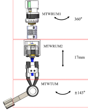
Figure 2.1: Design and Illustration of Ultrasonic Motors[14].
