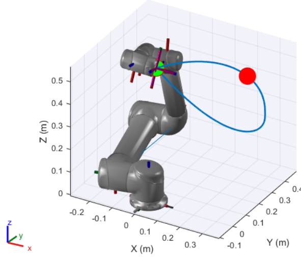
Figure 4.4: Lasso Gripper string loop is set at the end of UR5 robotic arm. The green point at the end of the robotic arm marks the position reachable by a rigid manipulator, while the red point indicates the furthest position on the string loop from the original point at the same robotic position.
