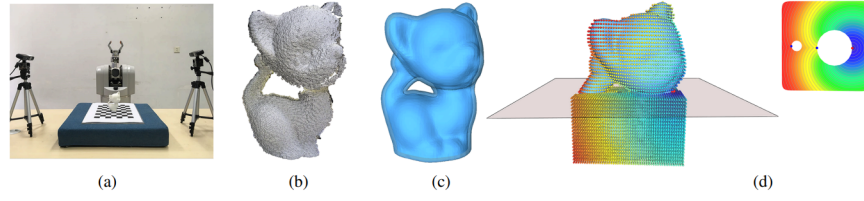
Figure 4.1: The caging loop calculating algorithm for Lasso Gripper [19]. (a) The setup of the depth reconstruction system (b) The Point cloud captured by depth camera directly. (c) A r-offset surface is built for defining the grasping space. (d) Two Morse saddle points (blue) are calculated to define the grasping loop.
