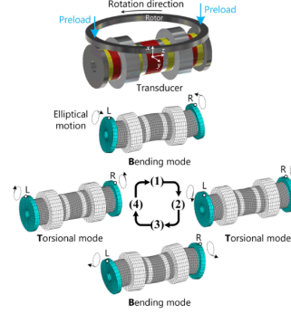
Figure 2.2: Bending and Torsion layouts of the Transducer[32].
