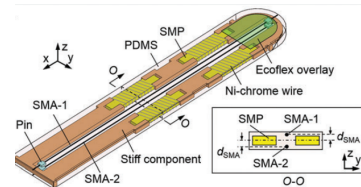
Figure 2.13: Shape Memory Alloy-Based Soft Gripper [31]
