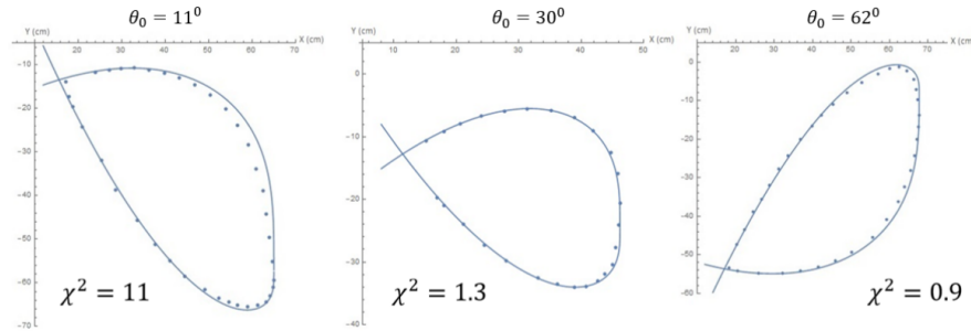
Figure 4.3: The string loop curve fitting of numerical theoretical solution with experimental profiles [1]. In this case, the linear mass \mu = 0.283 \pm 0.005 \text{ g} \cdot \text{m}^{-1} , the length of the string loop L = 160 \text{ cm} , shooting velocity v = 5.1 \text{ m} \cdot \text{s}^{-1} and several values of ejection pitch angle \theta_0 . A satisfactory fitting result with \chi^2 \leq 11 is obtained.
