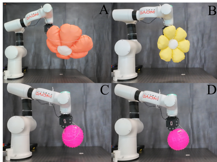
Figure 4.8: Validation of grasping ability with oversized objects: inflated balloons.
