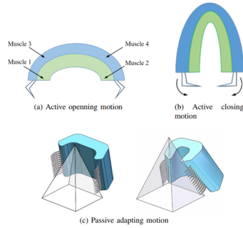
Figure 2.12: Bio-mechanism of inchworm's true leg [15]
