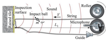
Figure 2.16: String shoot impact towards a wall [28]
