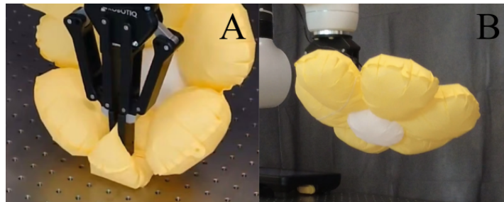
Figure 4.10: The inflated balloon is captured by the antipodal gripper. As a result of the concentrated stress applied, the balloon was severely deformed.
