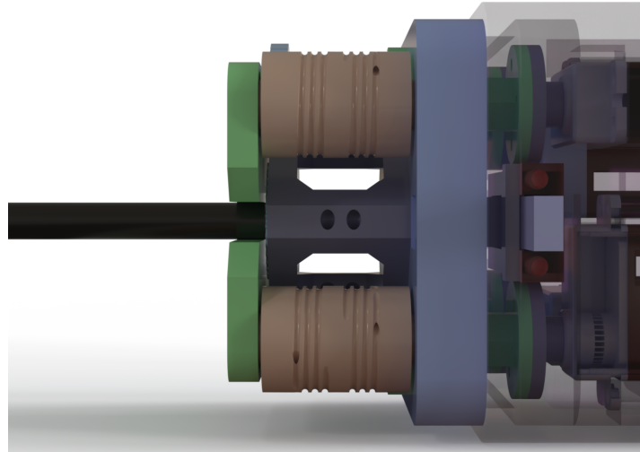
Figure 5.4: Reel Design and Winding Mechanism
