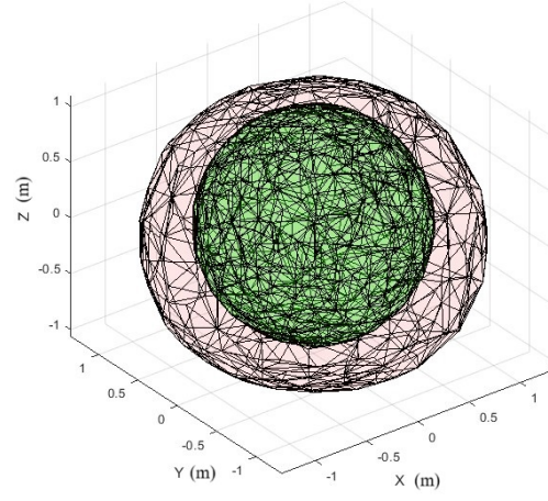
Figure 4.5: The initial robotic arm workspace is marked in green and extended Lasso Gripper workspace is marked in red.
