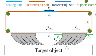
Figure 2.6: Belt Loop Actuated Adhesion Design [4]
