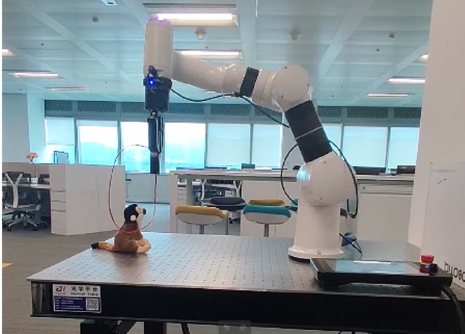
Figure 4.2: The illustration of the relative position of the string loop and the target object – an early test
