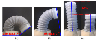
Figure 2.3: flexible fluidic actuators formed with granular to vary stiffness [23]
