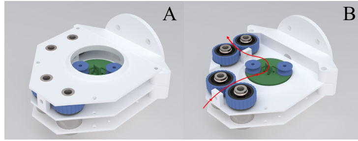
Figure 1.3: Prototype of the proposed Lasso Gripper.
