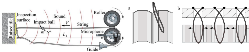
Figure 2.16: String shoot impact towards a wall [28]
