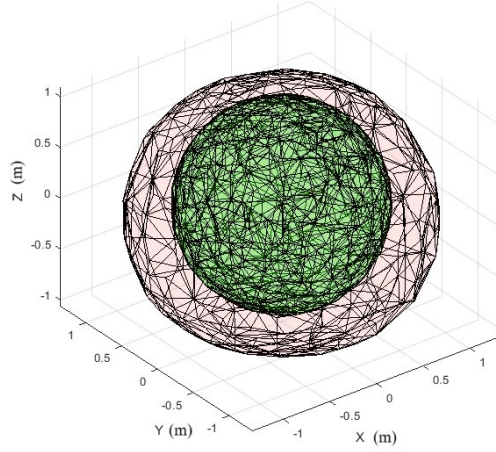
Figure 5.3: The initial robotic arm workspace is marked in green and extended Lasso Gripper workspace is marked in red.
