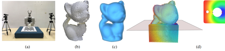
Figure 4.1: The caging loop calculating algorithm for Lasso Gripper [19]. (a) The setup of the depth reconstruction system (b) The Point cloud captured by depth camera directly. (c) A r-offset surface is built for defining the grasping space. (d) Two Morse saddle points (blue) are calculated to define the grasping loop.
