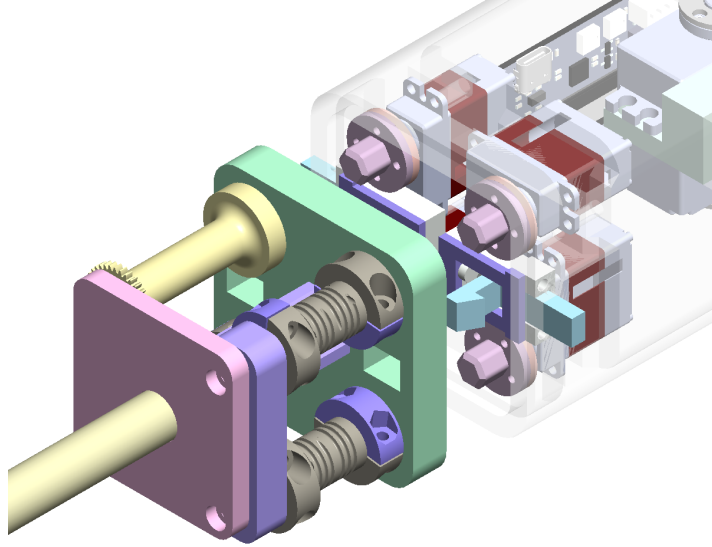
Figure 8.4: Motor Arrangement and Quick-Swap Mechanism
