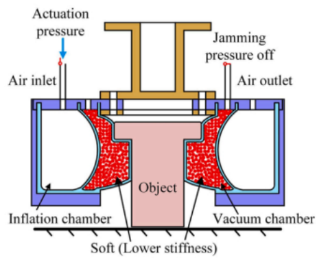
Figure 2.5: Pressurized the actuation chamber and adaptive grasping [10]
