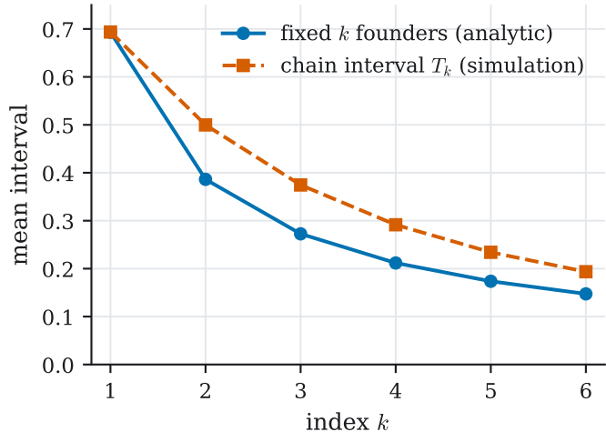
(b) inter-rupture intervals
