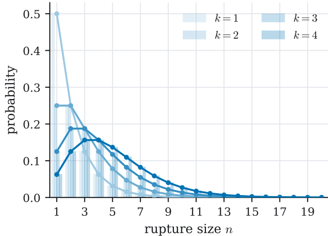
(a) rupture-size laws
