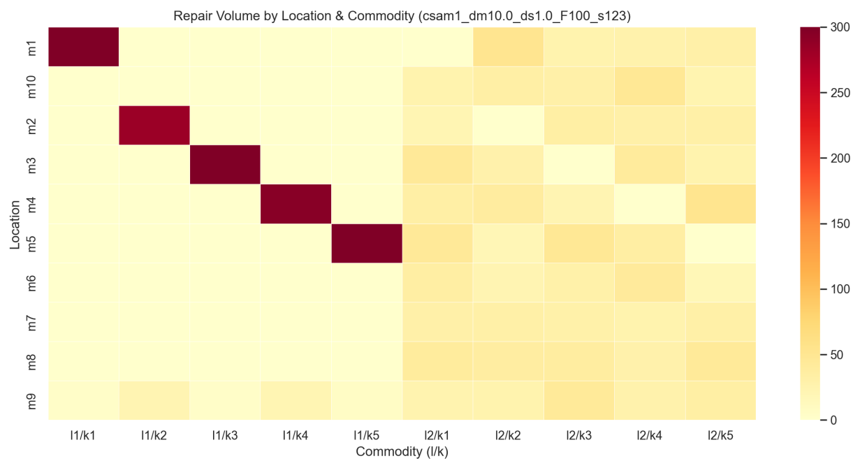
repair_heatmap_(csam1_dm10.0_ds1.0_F100_s123).png
