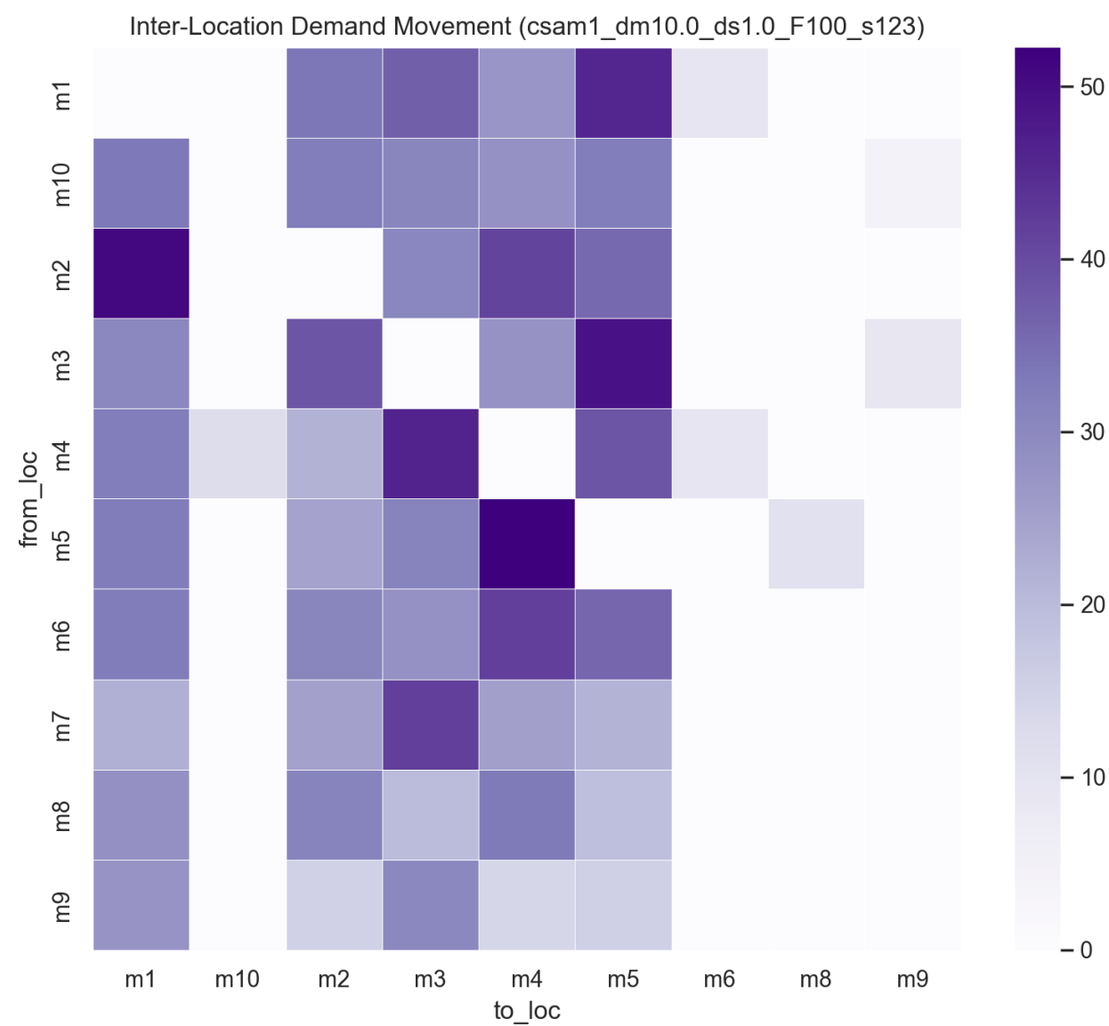
movement_heatmap_(csam1_dm10.0_ds1.0_F100_s123).png
