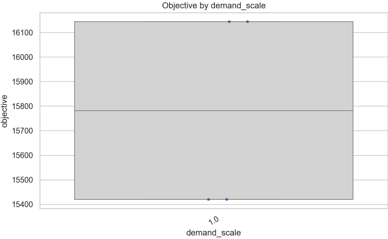
objective_by_demand_scale.png
