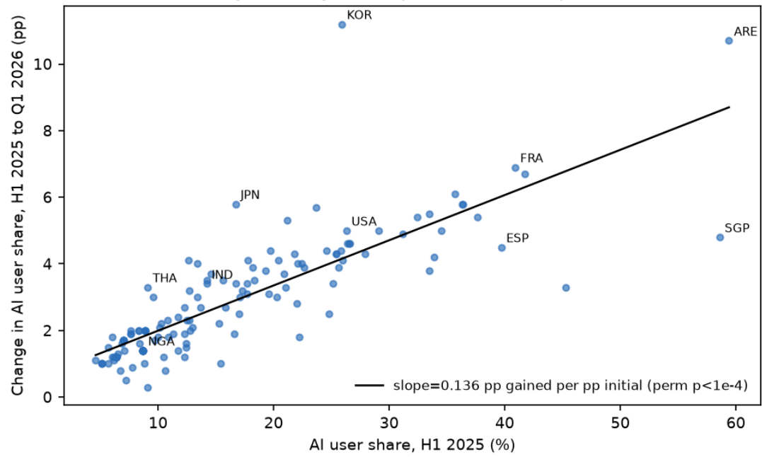
Absolute divergence: higher-adoption economies pull further ahead
