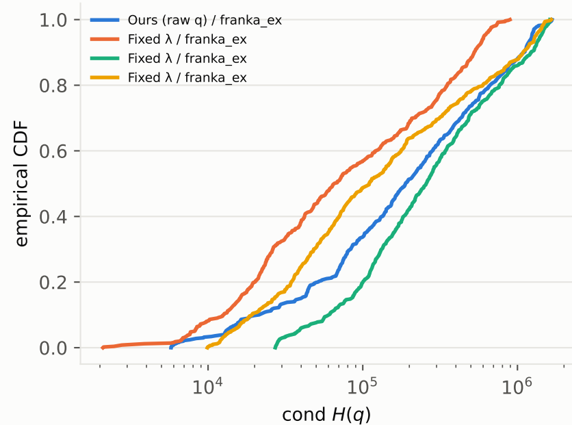
Inertia-matrix conditioning
