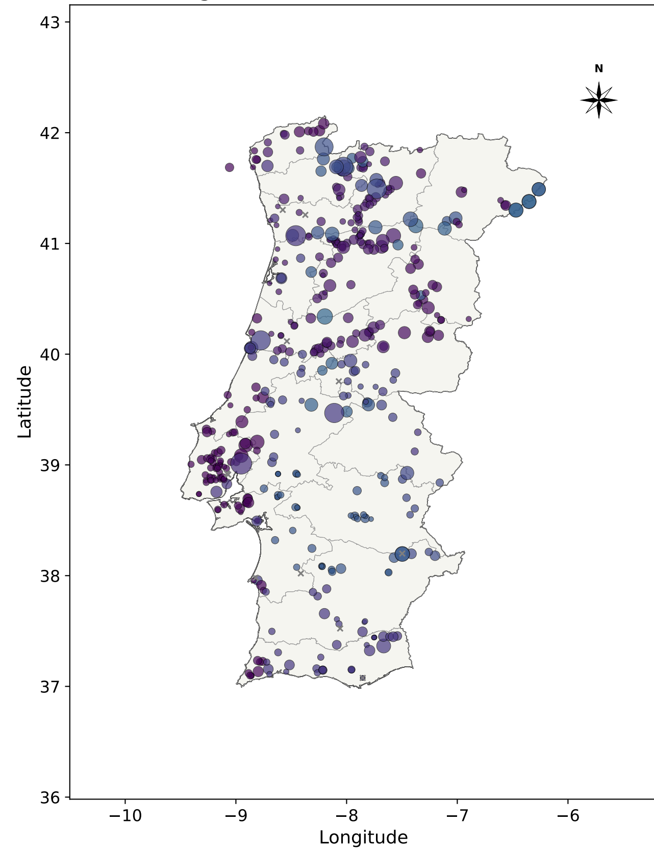
Portugal (Power Plants=439, excluded=11)
