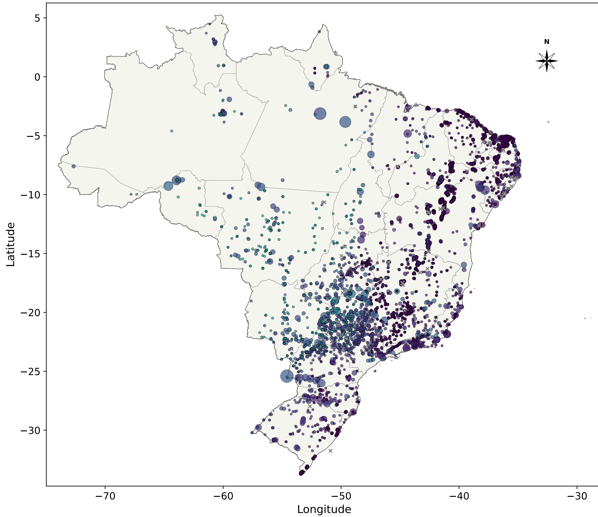
Brazil (Power Plants=5,178, excluded=97)
