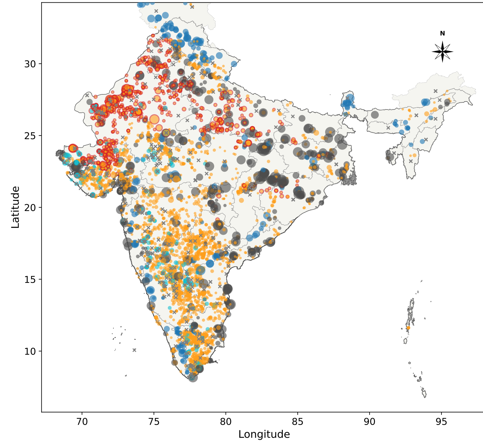
India (Power Plants=4,589, excluded=494)
