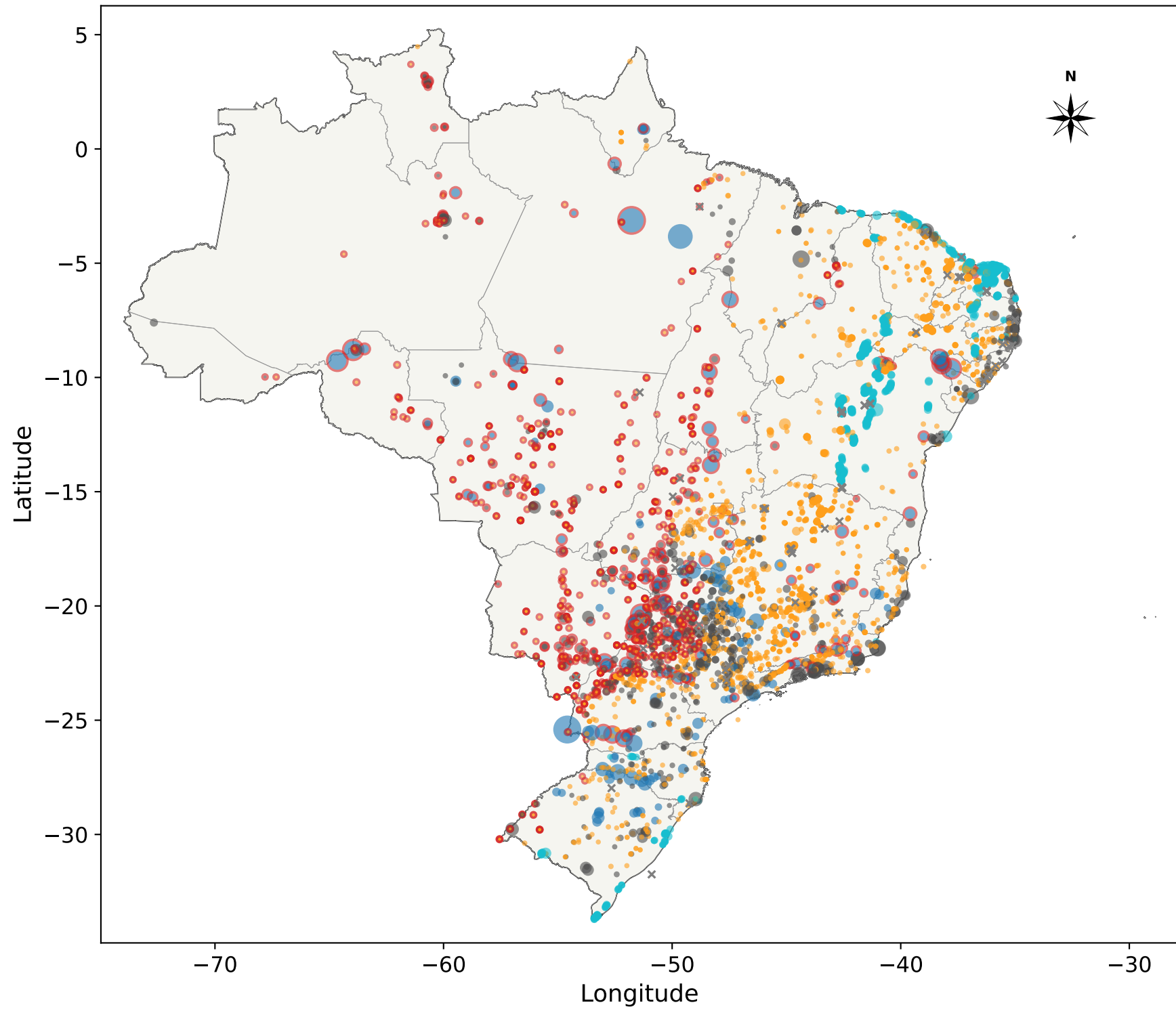
Brazil (Power Plants=5,178, excluded=97)
