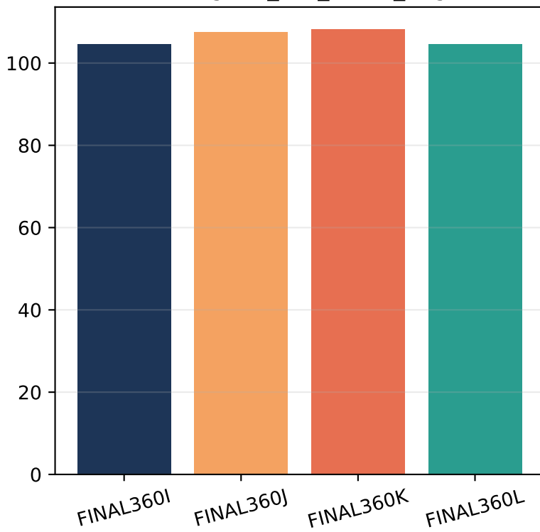
val signed_tdir_mean_deg
