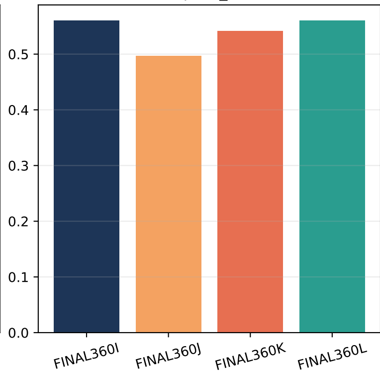
val path_ratio
