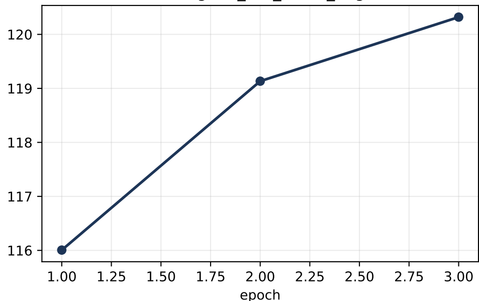
train loss
