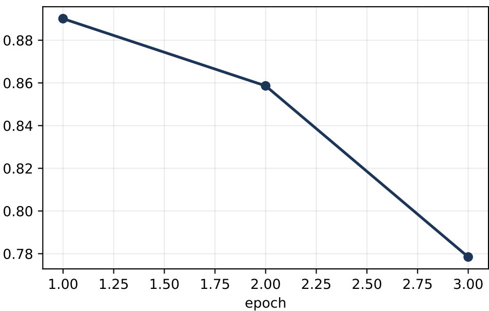
train loss
