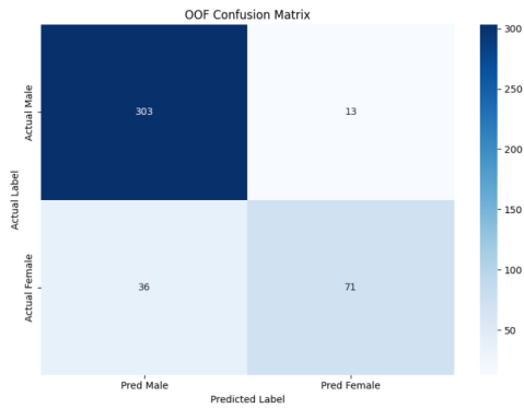
Figure 13. Confusion Matrix: VAE (Full Imputation). Increased noise leads to more misclassifications than MissForest.
