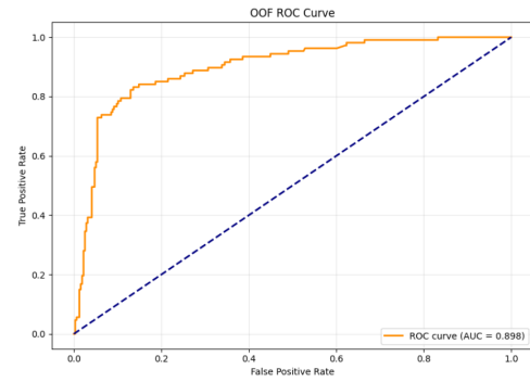
Figure 15. ROC Curve: MissForest (Numerical + Unknown). The model maintains robust discriminative power.
