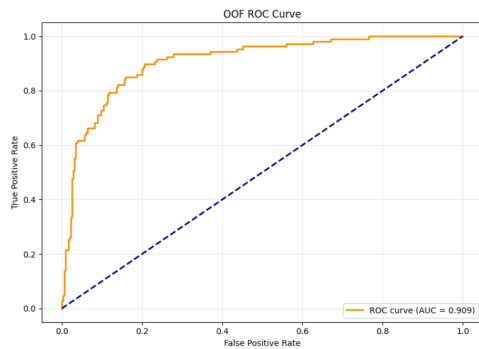
Figure 14. ROC Curve: Control Group. High AUC reflects stability on original distributions.
