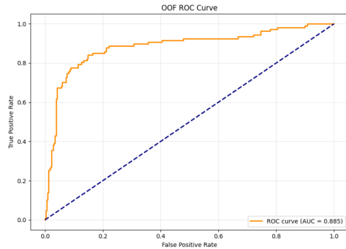
Figure 16. ROC Curve: VAE (Full Imputation). Shows a slight decrease in power due to noise on a small sample size.
