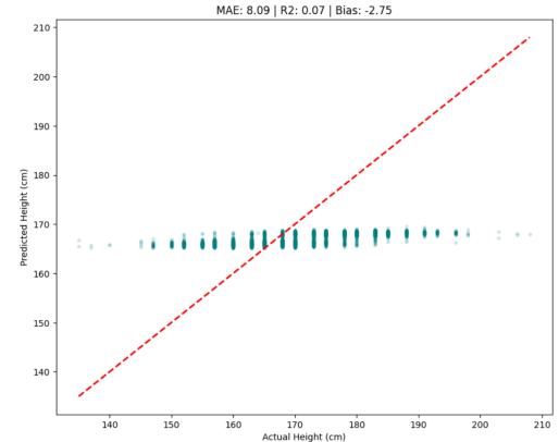
Figure 6: Median Imputation. Similar to the small dataset, it fails to capture any individual variance.
