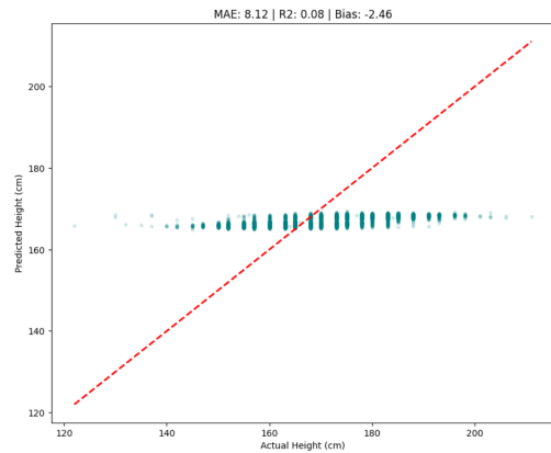
Figure 9: GAIN. The points are widely scattered and fail to align with the diagonal line, which visually explains the very low R^2 of 0.0791 and high MAE.
