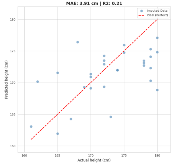
Figure 11. MissForest Imputation (Small Dataset).
