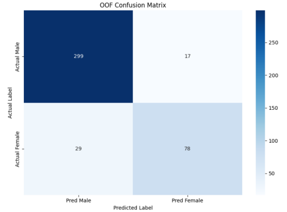
Figure 13. Confusion Matrix: MissForest (Numerical + Unknown).
