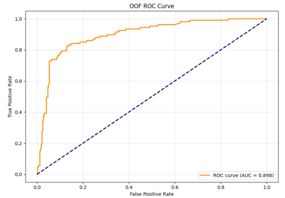
Figure 14. ROC Curve: MissForest (Numerical + Unknown).
