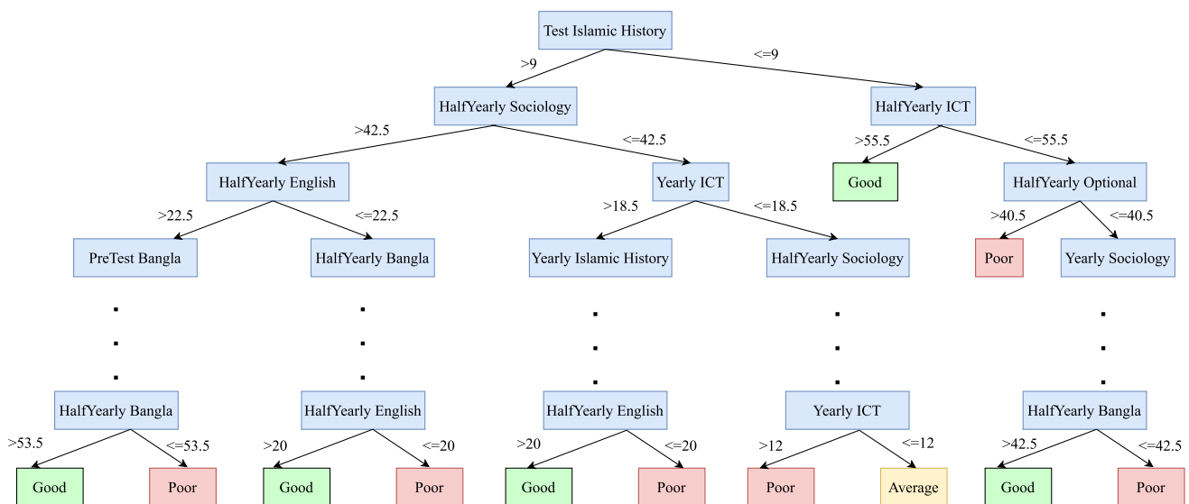
Fig. 3. Decision tree with Information Gain (Board GPA).
