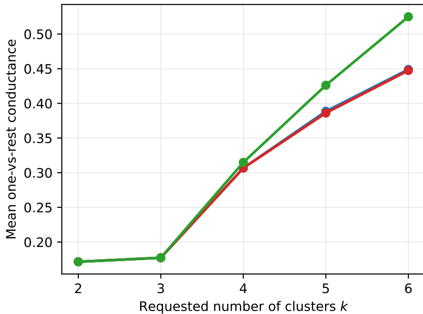
Conductance vs. k
