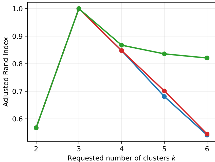
ARI vs. k
