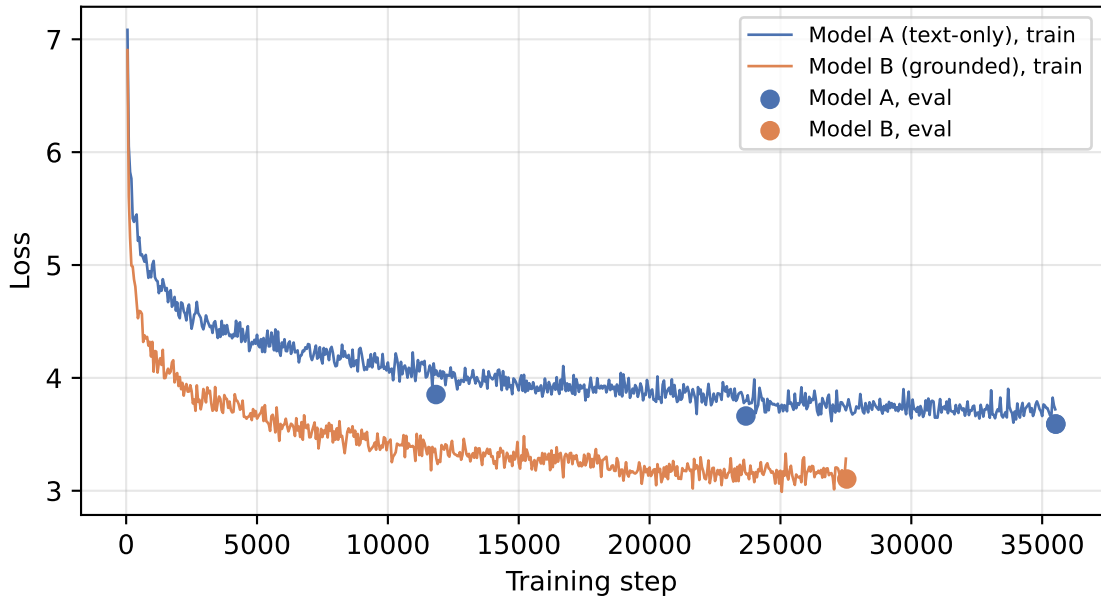
Training and evaluation loss over time
