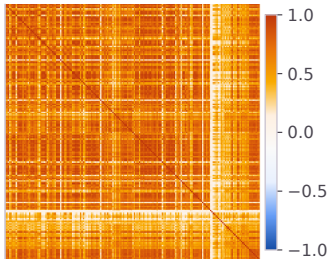
(a) Aggregate correlation
