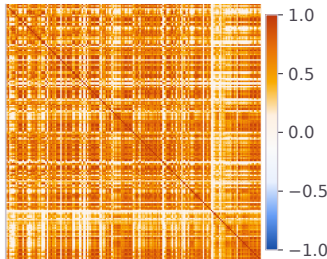
(b) Entry-channel correlation
