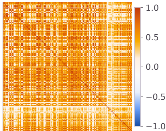
(c) Exit-channel correlation
