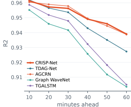
(c) R2
