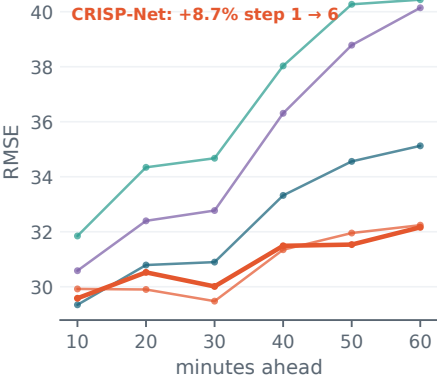
(a) RMSE
