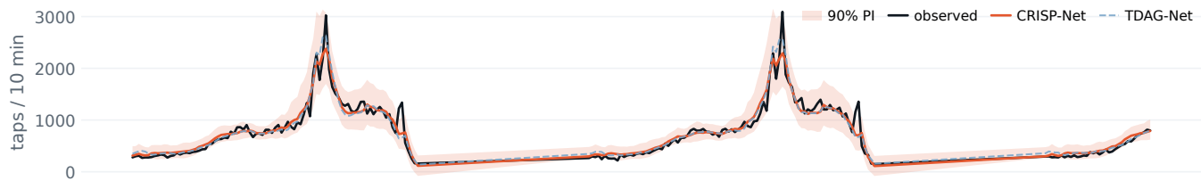
(b) Station 44 — entry, +10 min (WMAPE 17.3%)
