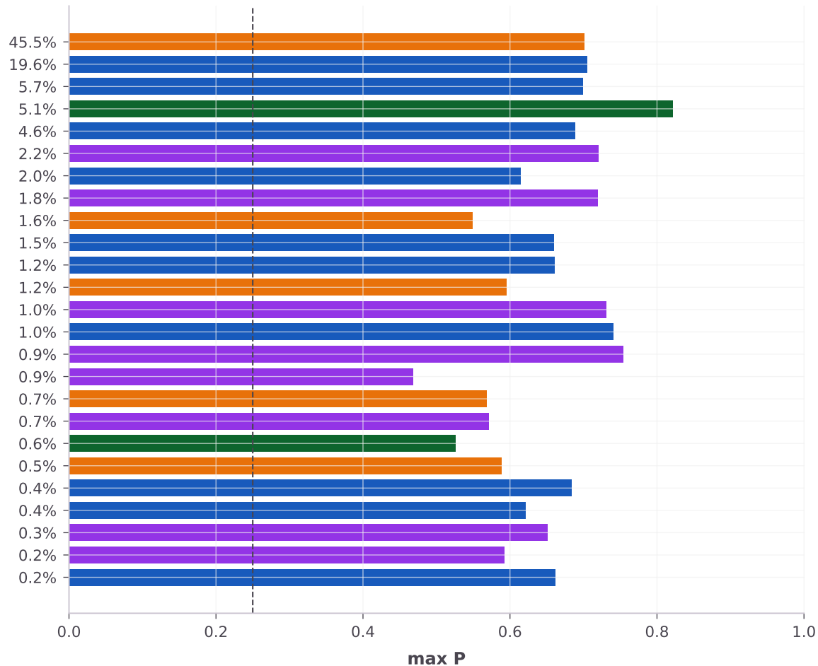
Assignment confidence
