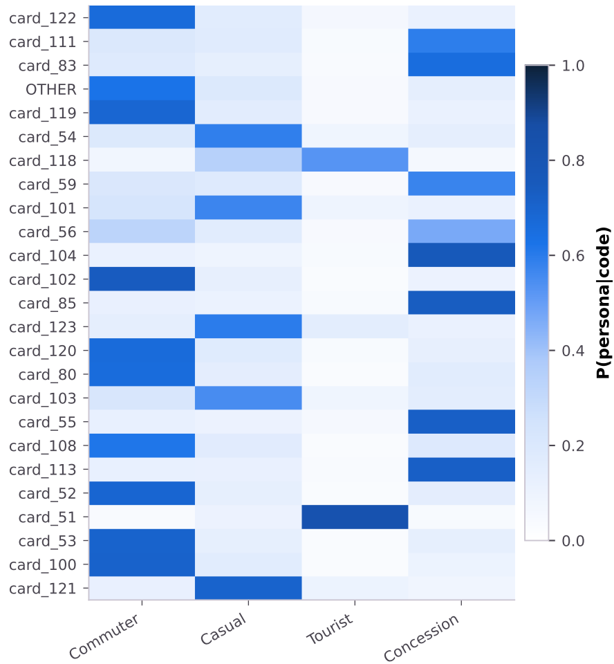
Soft-assignment prior P0
