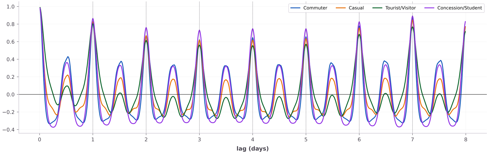
Persona flow autocorrelation
