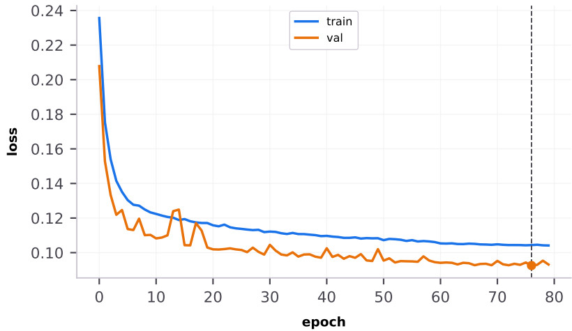
TDAG-Net w/o Adaptive
