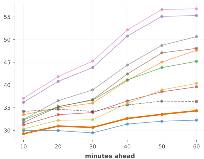
RMSE
