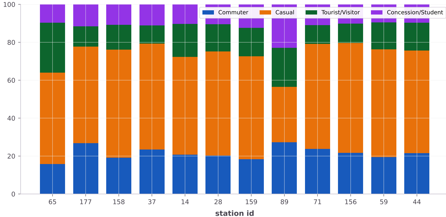
Event-peak persona composition
