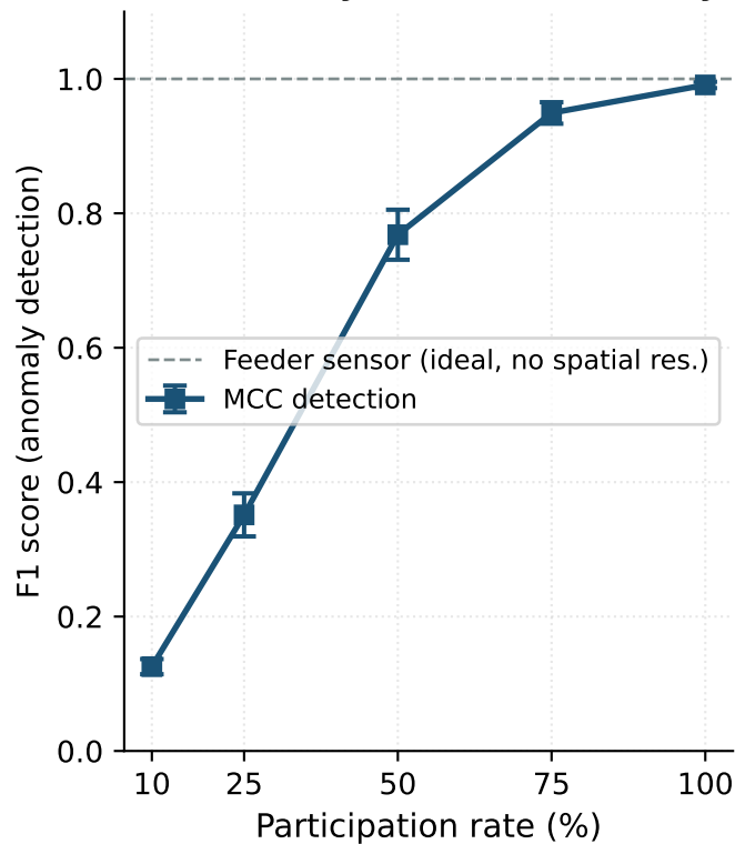
(b) Anomaly detection accuracy
