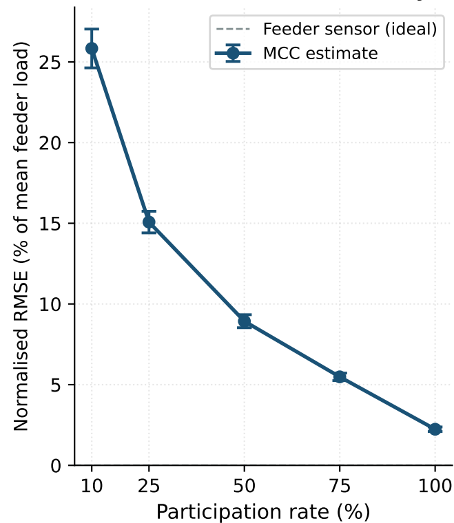
(a) Load estimation accuracy
