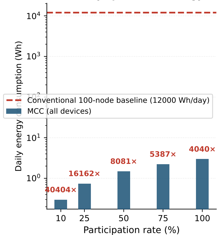
(c) Daily operational energy
