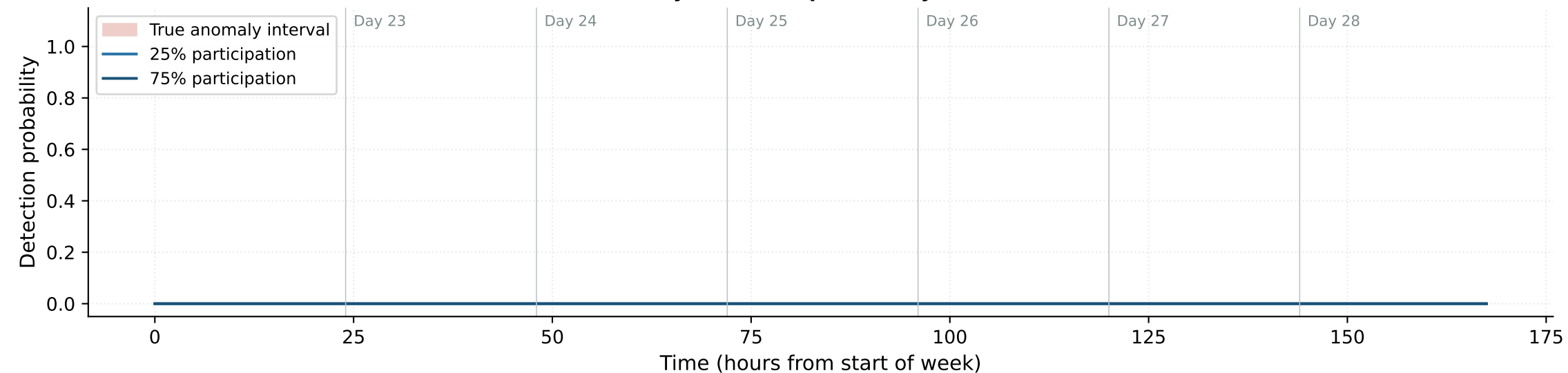
Anomaly detection probability (30 trials)
