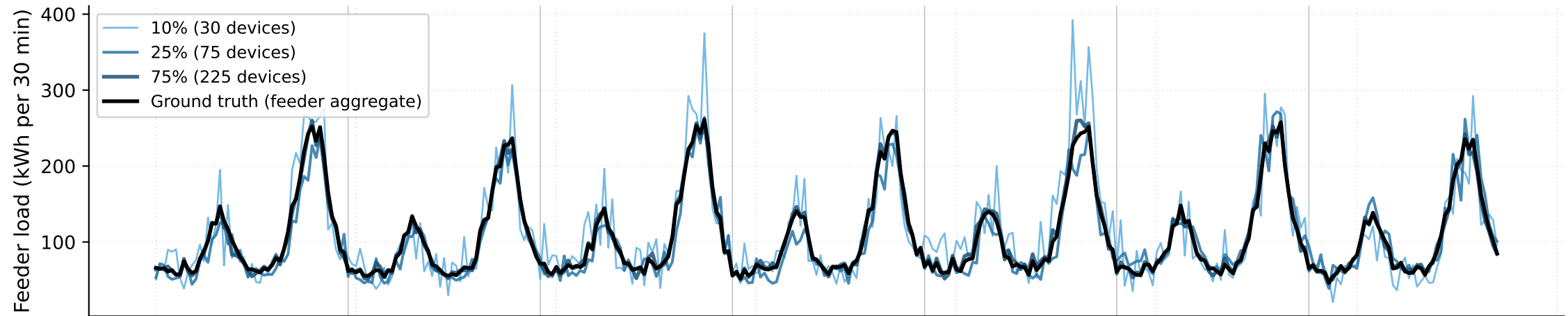
MCC load estimation — one-week excerpt
