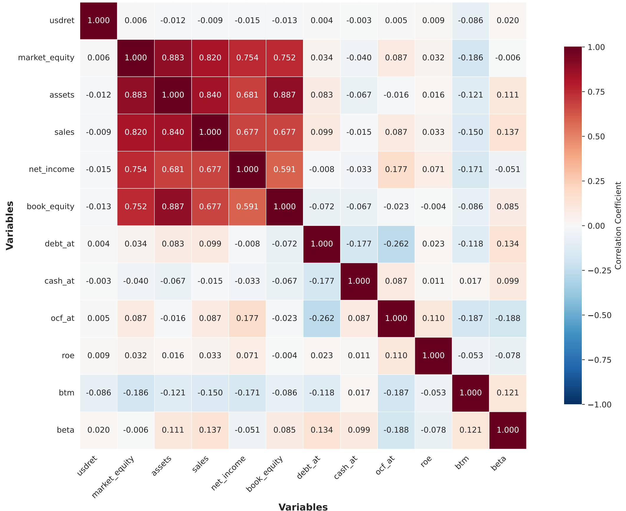
Correlation Heatmap: REIT Returns and Financial Variables (2000-2024)
