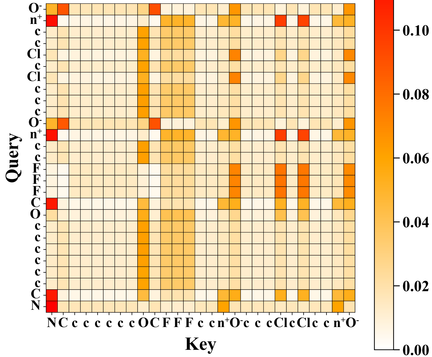
Attention Heatmap - Layer 2 Avg
