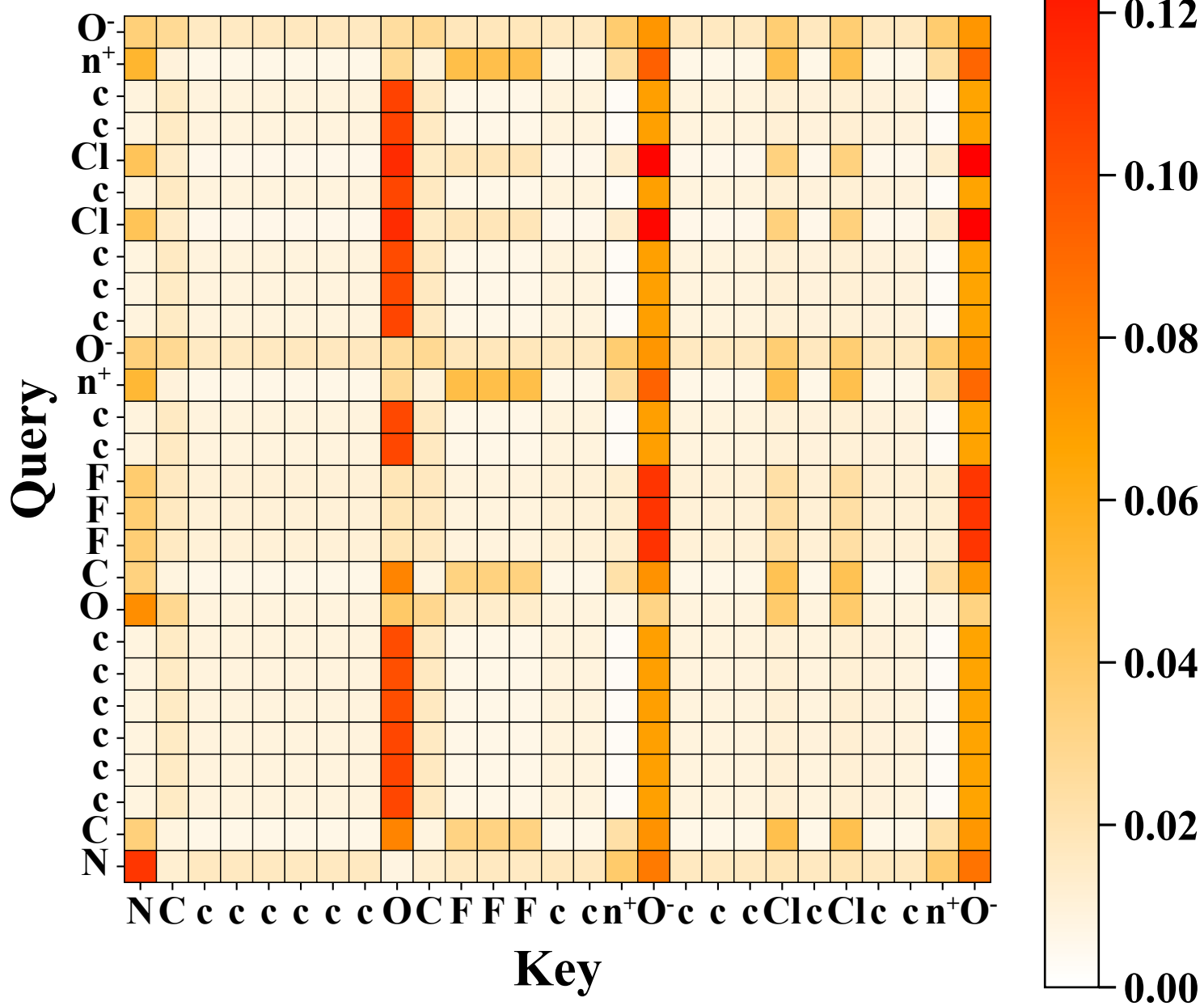
Attention Heatmap - Layer 3 Avg
