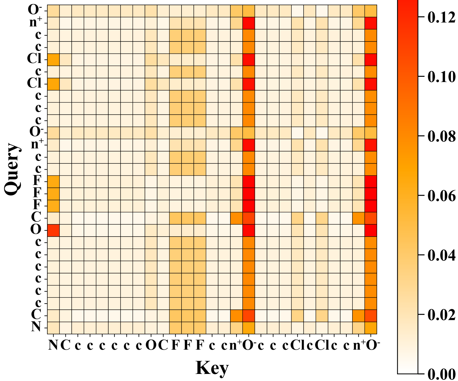
Attention Heatmap - Layer 4 Avg
