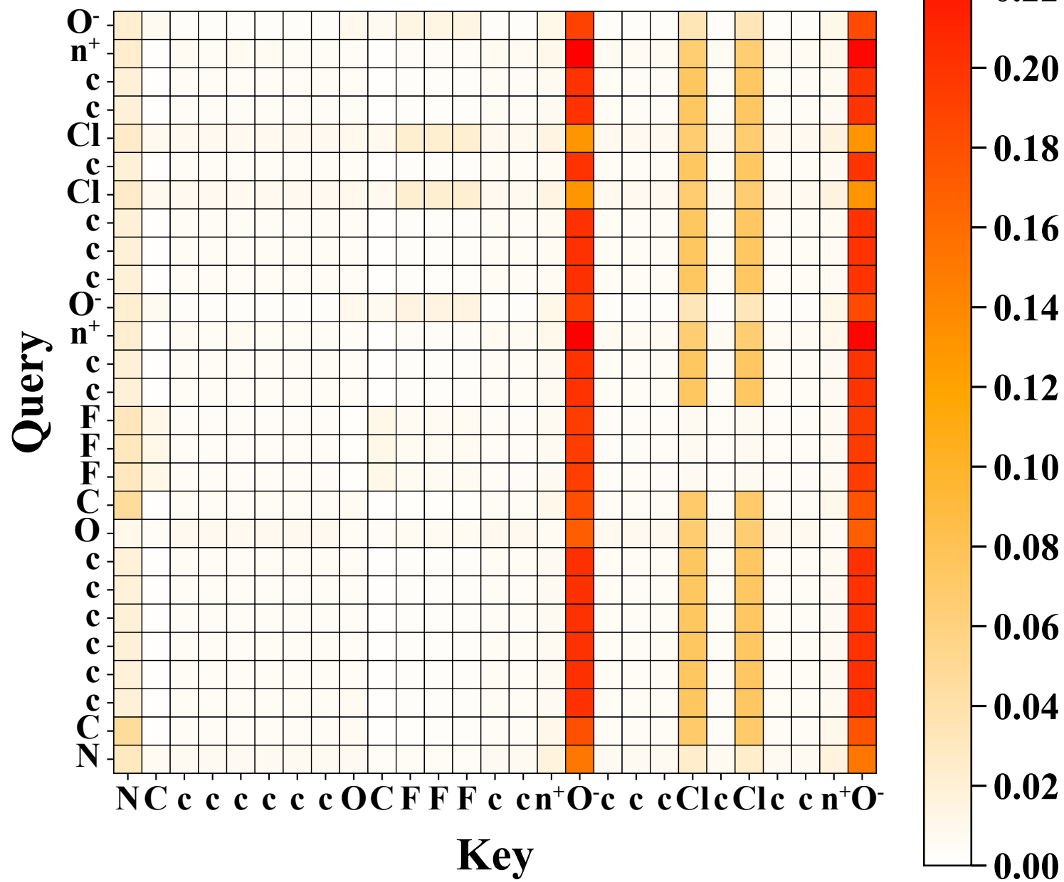
Attention Heatmap - Layer 6 Avg
