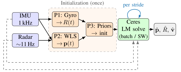
Fig. 1. System pipeline. Solid: initialization flow (P1–P3 seed the optimizer, run once). Dashed: raw sensor data fed as measurement factors. Blue: the sliding-window re-solve at each stride. Radar returns first pass a RANSAC ego-velocity prefilter (Section V-B) that rejects elevation-biased outliers before both P2 and the solver. MoCap supplies only the yaw heading prior (magnetometer surrogate) and RMSE evaluation.
