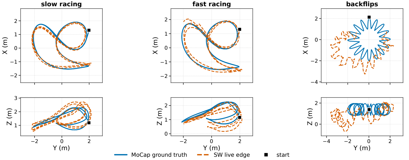
Fig. 2. Trajectory overlays for all three flights (columns): MoCap ground truth vs. the SW live edge, X-Y (top) and Y-Z (bottom) projections. Within each column both projections share a common Y range and metric scale (equal aspect, so loops keep their true shape); the scale differs between columns, so compare shapes rather than absolute sizes across columns. Start \blacksquare . Larger fast-racing deviations reflect higher dynamics ( \omega_{\max} = 9.1 \text{ rad/s} ); on backflips the residual \sim 6^\circ live orientation error attenuates the loop circles while the donut sweep and altitude are followed.
