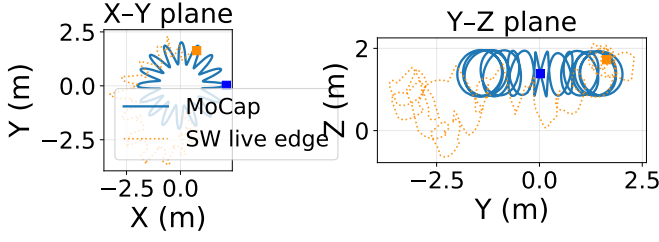
Fig. 2. backflips: MoCap ground truth (solid blue) and SW live edge (dotted orange; consistent prior, soft gate, elevation-bias correction, default RANSAC front-end). The batch estimate is omitted — at \Delta t_o=0.8 ms it is bistable (Sec. VII-B) and the SW live edge is the trustworthy result. X–Y and Y–Z projections; the vertical backflip maneuvers are visible in the Y–Z plane. Start marked \blacksquare . The estimate follows the overall donut sweep and altitude; the residual \sim 6^\circ live orientation error through flips attenuates the individual loop circles relative to ground truth.
