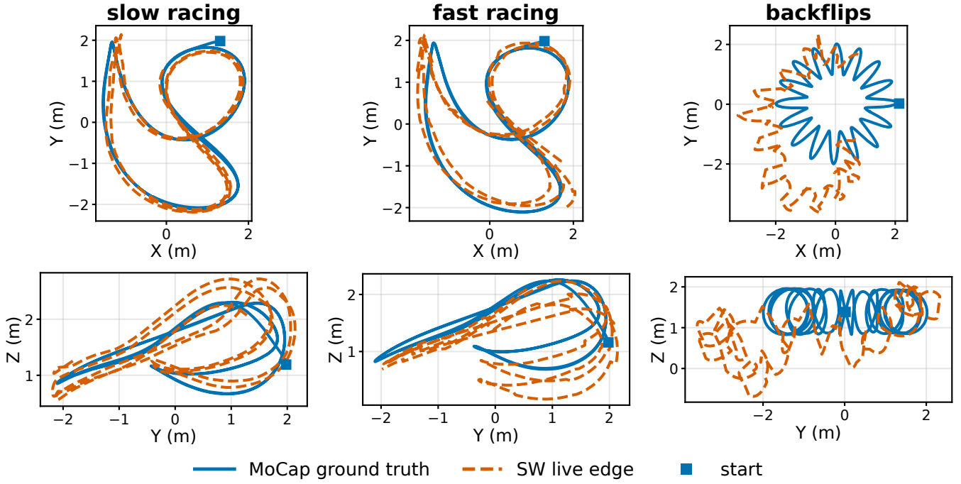
Fig. 3. Trajectory overlays for all three flights (columns): MoCap ground truth vs. the SW live edge, X-Y (top) and Y-Z (bottom) projections; start ■. Larger fast-racing deviations reflect higher dynamics ( \omega_{\max} = 9.1 \text{ rad/s} ); on backflips the residual \sim 6^\circ live orientation error attenuates the loop circles while the donut sweep and altitude are followed.
