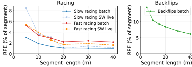
Fig. 5. KITT-style translational RPE (end-point displacement error as % of segment length) vs. accumulated GT distance. Left: racing bags, batch (solid) and SW live edge (dashed). Right: backflips batch.
