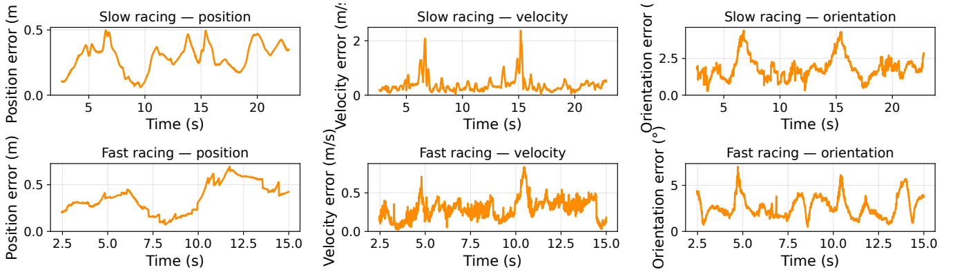
Fig. 4. SW live-edge (deployed) position, velocity, and orientation error vs. time for slow racing (top) and fast racing (bottom). Fast racing position error accumulates monotonically with trajectory length; velocity and orientation errors spike at high-speed, high-dynamics sections. Backflips omitted (flip-time GT mask gaps; Section VII-C).
