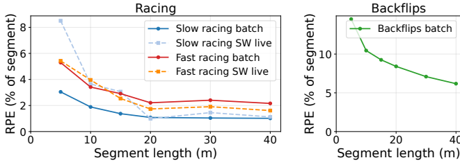
Fig. 5. KITTI-style translational RPE (end-point displacement error as % of segment length) vs. accumulated GT distance. Left: racing bags, batch (solid) and SW live edge (dashed). Right: backflips batch.
