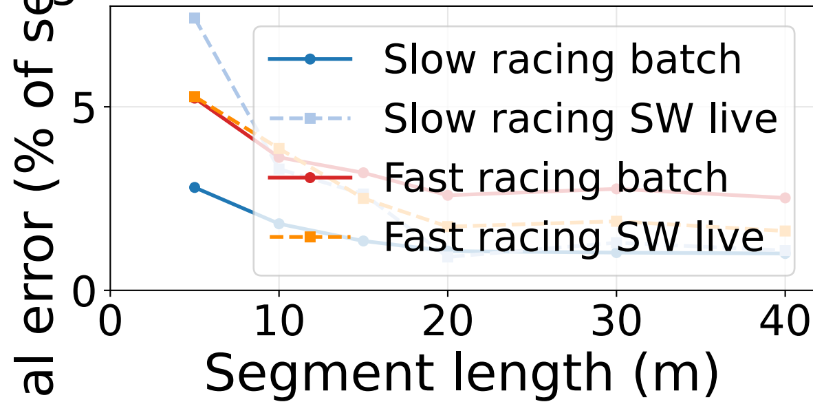
Racing maneuvers — KITTI translational RPE — KITTI translational RPE
