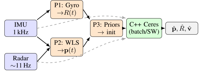
Fig. 1. System pipeline. Solid: initialization flow (P1–P3 seed the optimizer). Dashed: raw sensor data fed as measurement factors. Radar returns first pass a RANSAC ego-velocity prefilter (Sec. IV-C) that rejects elevation-biased outliers before both P2 and the solver. MoCap supplies only the yaw heading prior (magnetometer surrogate) and RMSE evaluation.
