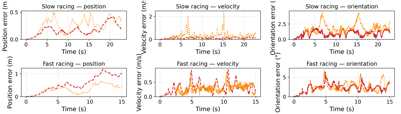
Fig. 4. Position, velocity, and orientation error vs. time for slow racing (top) and fast racing (bottom). Batch estimate (red dashed) and SW live edge (orange dotted). Fast racing position error accumulates monotonically with trajectory length; velocity and orientation errors spike at high-speed, high-dynamics sections. Backflips omitted (flip-time GT mask gaps, bistable batch reference; Section VII-C).
