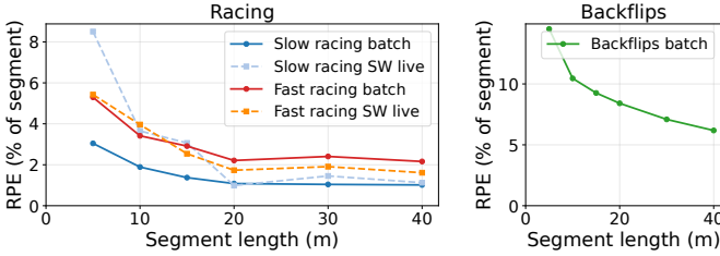
Fig. 5. KITTI-style translational RPE (end-point displacement error as % of segment length) vs. accumulated GT distance. Left: racing bags — batch (solid) and SW live edge (dashed). Right: backflips batch.
