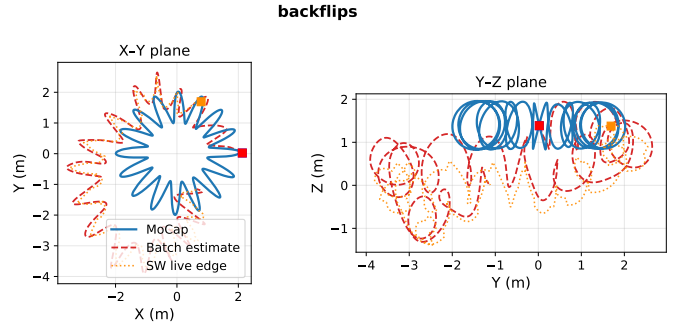
Fig. 7. backflips: MoCap ground truth (solid blue), batch estimate ( \Delta t_o = 0.8 ms, dashed red), SW live edge (consistent prior, soft gate, elevation-bias correction; dotted orange). X–Y and Y–Z projections; the vertical backflip maneuvers are visible in the Y–Z plane. Start marked ■. The estimate follows the overall donut sweep and altitude; the residual \sim 9^\circ orientation error through flips attenuates the individual loop circles relative to ground truth.
