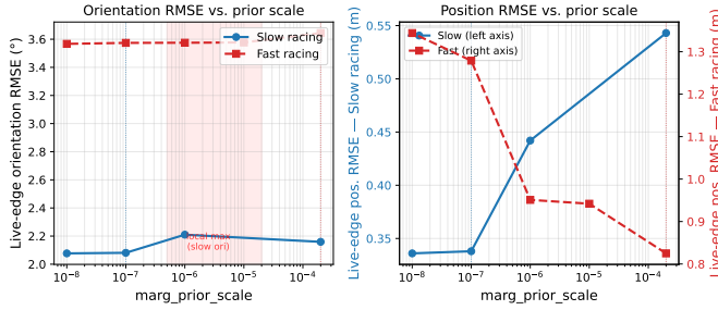
Fig. 8. Live-edge orientation (left) and position (right, dual y-axes) RMSE vs. marg_prior_scale . Orientation (left): slow racing shows a local maximum at 10^{-6} ; fast racing orientation is insensitive to scale. Position (right): slow racing worsens monotonically with increasing scale while fast racing improves sharply — the two bags require opposite scale regimes.
