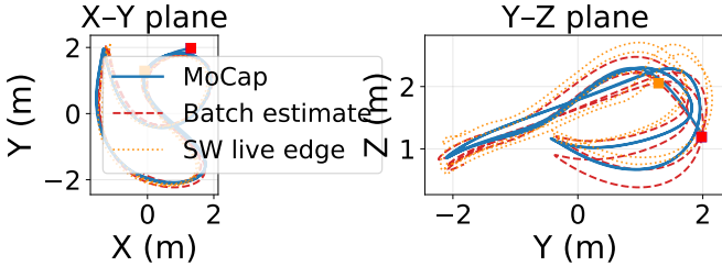
Fig. 3. slow_racing : MoCap ground truth (solid blue), batch estimate (dashed red), SW live edge (dotted orange). X–Y and Y–Z projections; start marked ■.
