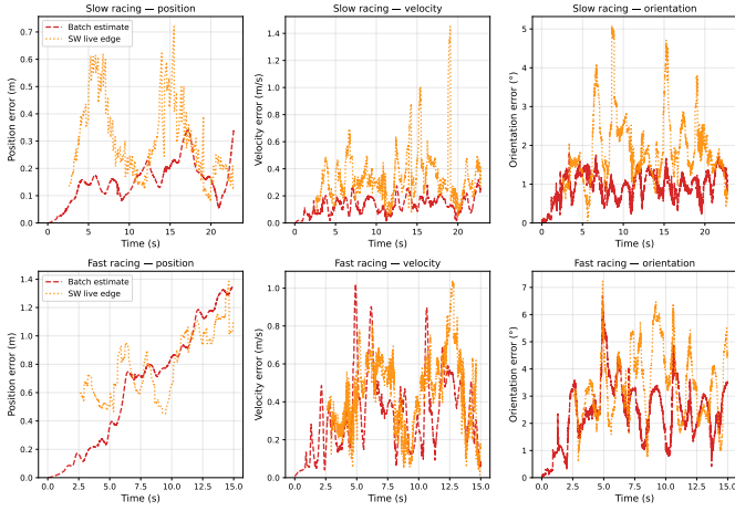
Fig. 5. Position, velocity, and orientation error vs. time for slow racing (top) and fast racing (bottom). Batch estimate (red dashed) and SW live edge (orange dotted). Fast racing position error accumulates monotonically with trajectory length; velocity and orientation errors spike at high-speed, high-dynamics sections.
