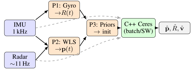
Fig. 1. System pipeline. Solid: initialization flow (P1–P3 seed the optimizer). Dashed: raw sensor data fed as measurement factors. MoCap used only for RMSE evaluation.
