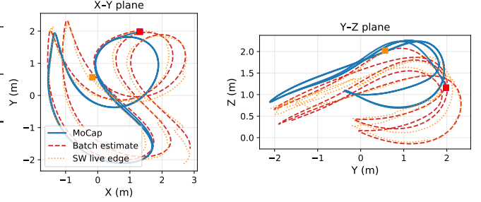
Fig. 4. fast_racing : MoCap ground truth (solid blue), batch estimate (dashed red), SW live edge (dotted orange). X–Y and Y–Z projections; start marked ■. Larger deviations reflect higher dynamics ( \omega_{\text{max}} = 9.1 rad/s) compared to slow racing.
