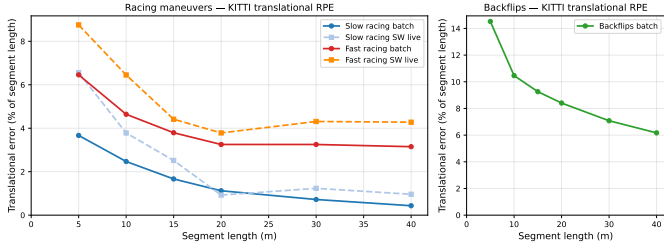
Fig. 6. KITTI-style translational RPE (end-point displacement error as % of segment length) vs. accumulated GT distance. Left: racing bags — batch (solid) and SW live edge (dashed). Right: backflips batch. Errors decrease at longer segments because the global optimizer integrates more sensor data; at short segments the 11 Hz radar provides limited constraints.
