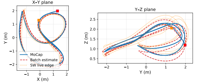
Fig. 3. slow_racing : MoCap ground truth (solid blue), batch estimate (dashed red), SW live edge (dotted orange). X–Y and Y–Z projections; start marked ■.
