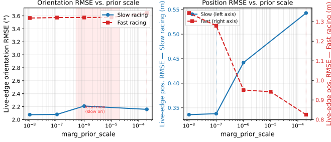
Fig. 8. Live-edge orientation (left) and position (right, dual y-axes) RMSE vs. \text{marg\_prior\_scale} . Orientation (left): slow racing shows a local maximum at 10^{-6} ; fast racing orientation is insensitive to scale. Position (right): slow racing worsens monotonically with increasing scale while fast racing improves sharply — the two bags require opposite scale regimes.
