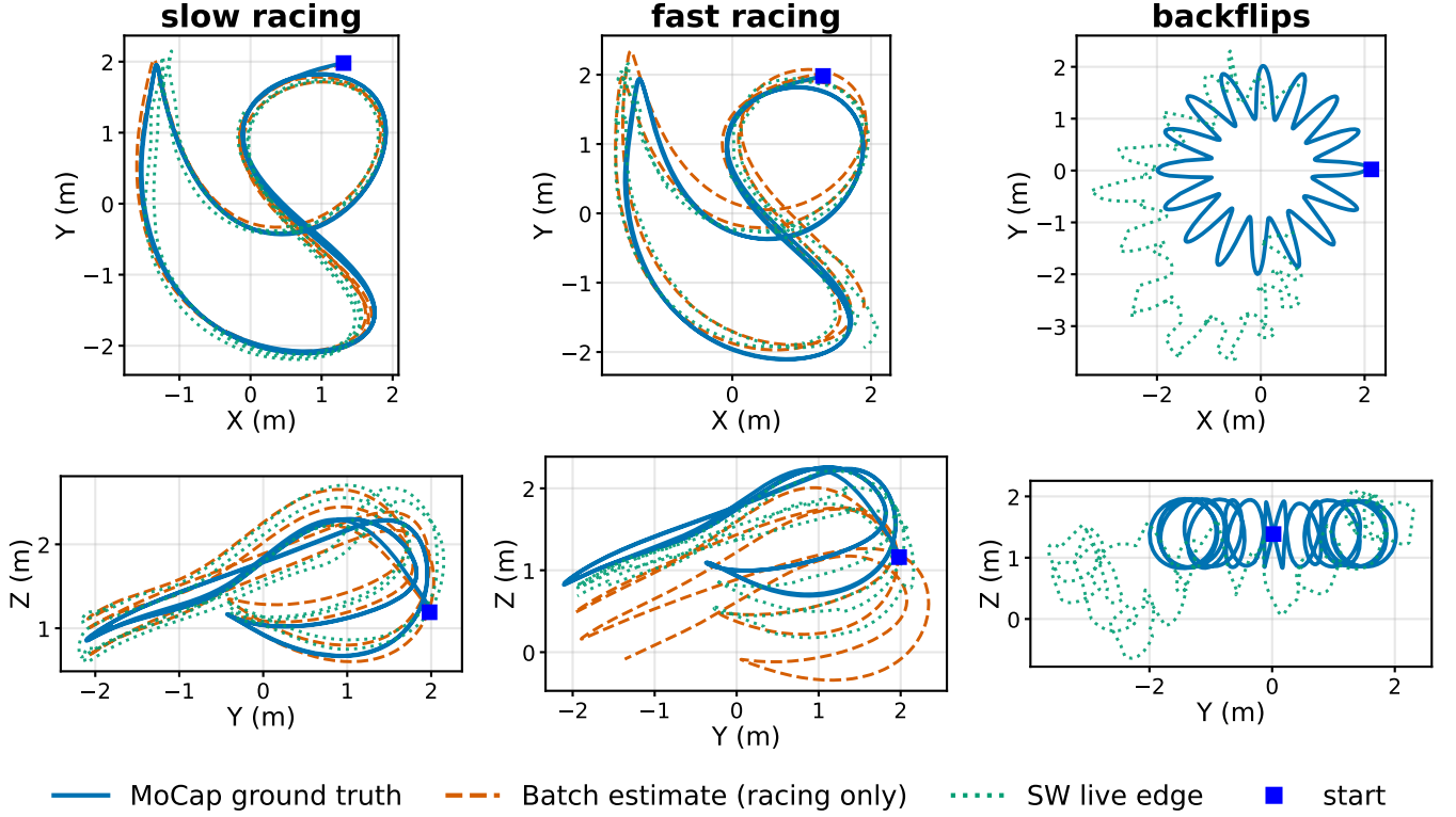
Fig. 1. Trajectory overlays for all three flights (columns), X-Y (top) and Y-Z (bottom) projections; start ■. Larger fast-racing deviations reflect higher dynamics ( \omega_{\max} = 9.1 rad/s). The backflips batch estimate is omitted (bistable, Sec. VII-B); its residual \sim 6^\circ live orientation error attenuates the loop circles while the donut sweep and altitude are followed.
