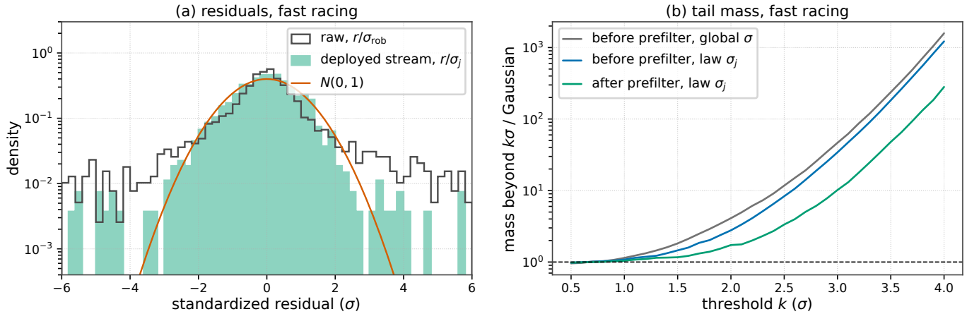
Fig. 5. The residual distribution before and after the front end (fast racing). (a) Standardized residuals on a log density scale: the raw stream in units of its \sigma_{\text{rob}} (grey) and the retained, non-aliased returns, each residual in units of its own \sigma_j (green), against N(0, 1) . Aliased returns are weighted as their own population and are not in the green stream. (b) Tail mass beyond k\sigma relative to a Gaussian, for the non-aliased returns before the prefilter with one global \sigma (grey) and with the per-return law \sigma_j (blue), and for the returns after the prefilter with the law (green). Together they reduce the excess by an order of magnitude. Per-return normalization mainly reduces the excess between 1.5\sigma and 3\sigma ; the blue and grey curves converge beyond 3.5\sigma . The prefilter reduces the remaining far tail.
