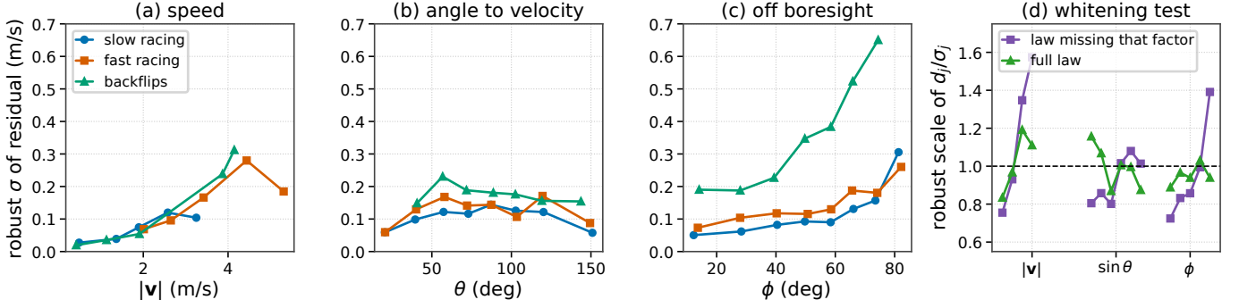
Fig. 4. The per-return noise law. (a–c) Robust width of the within-frame deviations binned by platform speed |\mathbf{v}| , by the angle \theta between ray and velocity, and by the angle \phi off boresight, for the three flights: the three trends of (7) are visible before fitting. (d) Model check on fast racing: robust scale of the normalized deviation d_j/\sigma_j binned along each input, for the full law (green) and the law missing the corresponding factor (purple). The expected scale is approximately 1; each missing factor leaves a trend along its own input.
