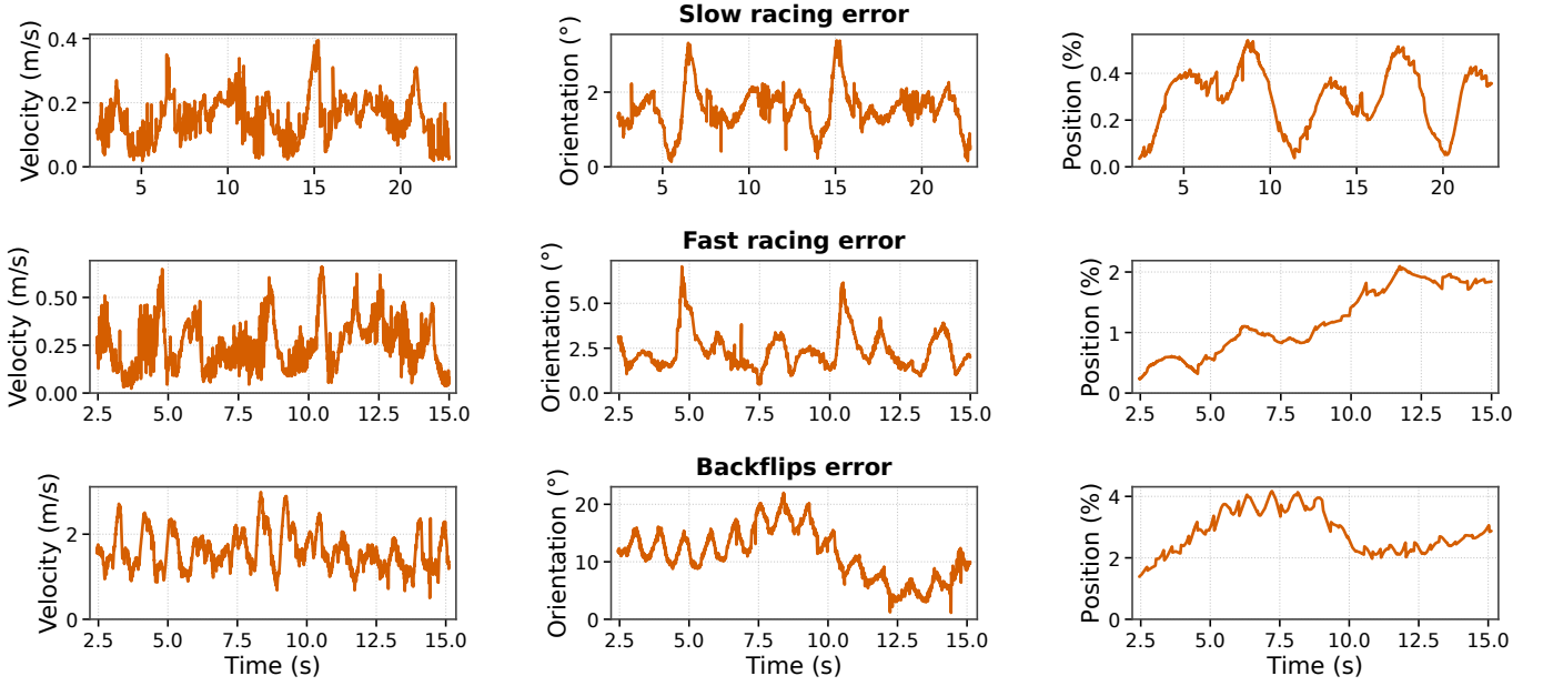
Fig. 7. Live-edge velocity, orientation, and position error (the last in percent of the flight's path length, the unit of the drift metric) vs. time for slow racing (top), fast racing (middle), and backflips (bottom). Velocity and orientation errors spike at high-speed, high-dynamics sections. Fast-racing position error accumulates with trajectory length. Backflip errors grow step-wise during the flips, where the radar measurement model degrades (Section IX-C).
