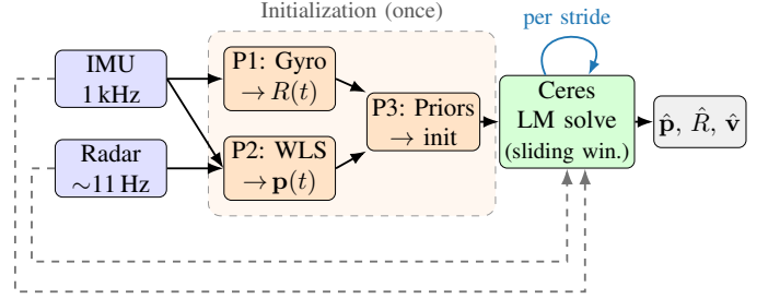
Fig. 2. System pipeline. Solid: initialization flow (P1–P3 seed the optimizer, run once). Dashed: raw sensor data fed as measurement factors. Blue: the sliding-window re-solve at each stride. Radar returns pass a RANSAC ego-velocity prefilter (Section VI-C) first. MoCap supplies only the yaw heading prior (magnetometer surrogate) and RMSE evaluation.
