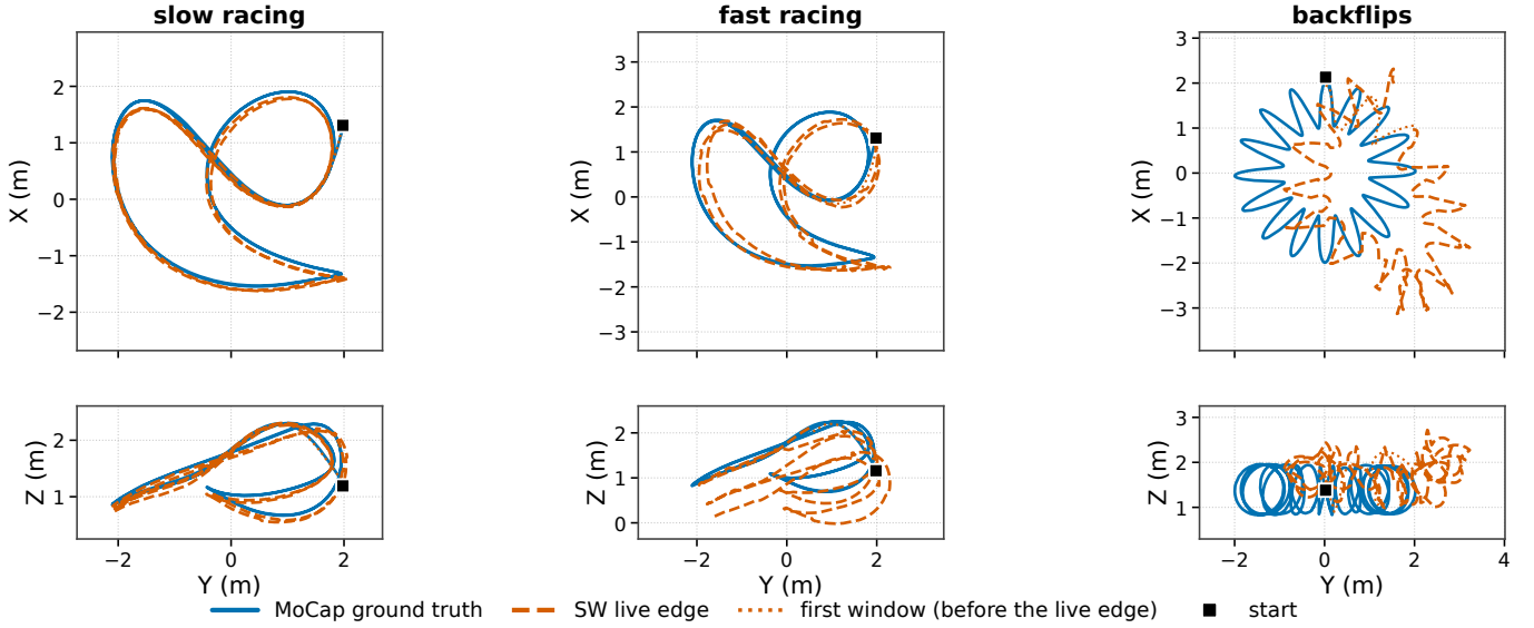
Fig. 6. Trajectory overlays for all three flights (columns): MoCap ground truth vs. the sliding-window live edge, X-Y (top) and Y-Z (bottom) projections. Within each column both projections share a common Y range and metric scale (equal aspect, so loops keep their true shape). The scale differs between columns. Start ■, the dotted lead-in is the first window’s estimate, available only once that window has been solved (the smoother needs one complete 3 s window), so it is not a live output at those timestamps. It starts on the ground truth by the start-anchored alignment. The backflip flight circles in the horizontal plane while looping in the vertical plane. Its position drifts through the flips (2.9% of the path) while the loops remain visible in the orientation estimate (Section IX-C).
