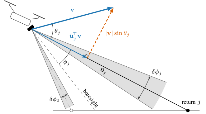
Fig. 3. Geometry behind the per-return law (Eq. (7)) in side view. The platform moves with velocity \mathbf{v} past static scene points. Return j is the ray of direction \hat{\mathbf{u}}_j from the radar to one of them. The sensor reads only the along-ray part of the velocity, the Doppler v_D = -\hat{\mathbf{u}}_j^\top \mathbf{v} (positive for a receding target, so negative here). A bearing error swings the ray about the radar (grey cones) and leaves its length unchanged, so to first order it projects only the transverse velocity, of magnitude |\mathbf{v}| \sin \theta_j , into the Doppler residual. \theta_j is the angle between the ray and \mathbf{v} . The angular width of the cone grows off the boresight (dashed: the sensor x axis, mounted 27.5^\circ below the body’s forward axis), from about \delta\phi_0 near the boresight to \delta\phi_j = \delta\phi_0 / \cos \phi_j at the off-boresight angle \phi_j . This widening follows from the angle FFT’s uniform binning in the direction cosine \sin \phi .
