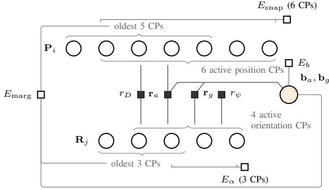
Fig. 1. Factor graph of one measurement time t . Circles are variables (position control points (CPs) \mathbf{P}_i , orientation control points \mathbf{R}_j , the shared IMU bias); filled squares are measurement factors, open squares the regularizers and the priors. Each factor at time t touches exactly the 6 active position CPs and/or the 4 active orientation CPs (braces): the radar Doppler factor r_D couples both splines (one such factor per return; the returns of a frame are stacked into one block, Section VI-C), the accelerometer \mathbf{r}_a both splines plus the bias, the gyroscope \mathbf{r}_g the orientation spline plus the bias, the heading factor r_\psi the orientation spline only. The minimum-snap regularizer E_{\text{snap}} spans 6 consecutive position CPs and the angular-acceleration regularizer E_\alpha 3 consecutive orientation CPs; the bias prior E_b anchors the bias to its pre-flight value (Section VI-A); the marginalization prior E_{\text{marg}} binds the window's oldest N-1 control points of each spline and the bias (Section VI-F). Not drawn: the priors of the first window (Section VI-E). Each row runs forward in time, but the two grids differ (40 and 16 ms), so horizontal positions are not aligned across rows.
