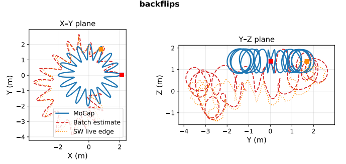
Fig. 7. backflips: MoCap ground truth (solid blue), batch estimate ( \Delta t_o=0.8 ms, dashed red), SW live edge (consistent prior, soft gate, elevation-bias correction; dotted orange). X–Y and Y–Z projections; the vertical backflip maneuvers are visible in the Y–Z plane. Start marked \blacksquare . The estimate follows the overall donut sweep and altitude; the residual \sim 9^\circ orientation error through flips attenuates the individual loop circles relative to ground truth.
